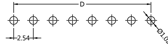
Recommended P.C.B Layout(±0.05)
